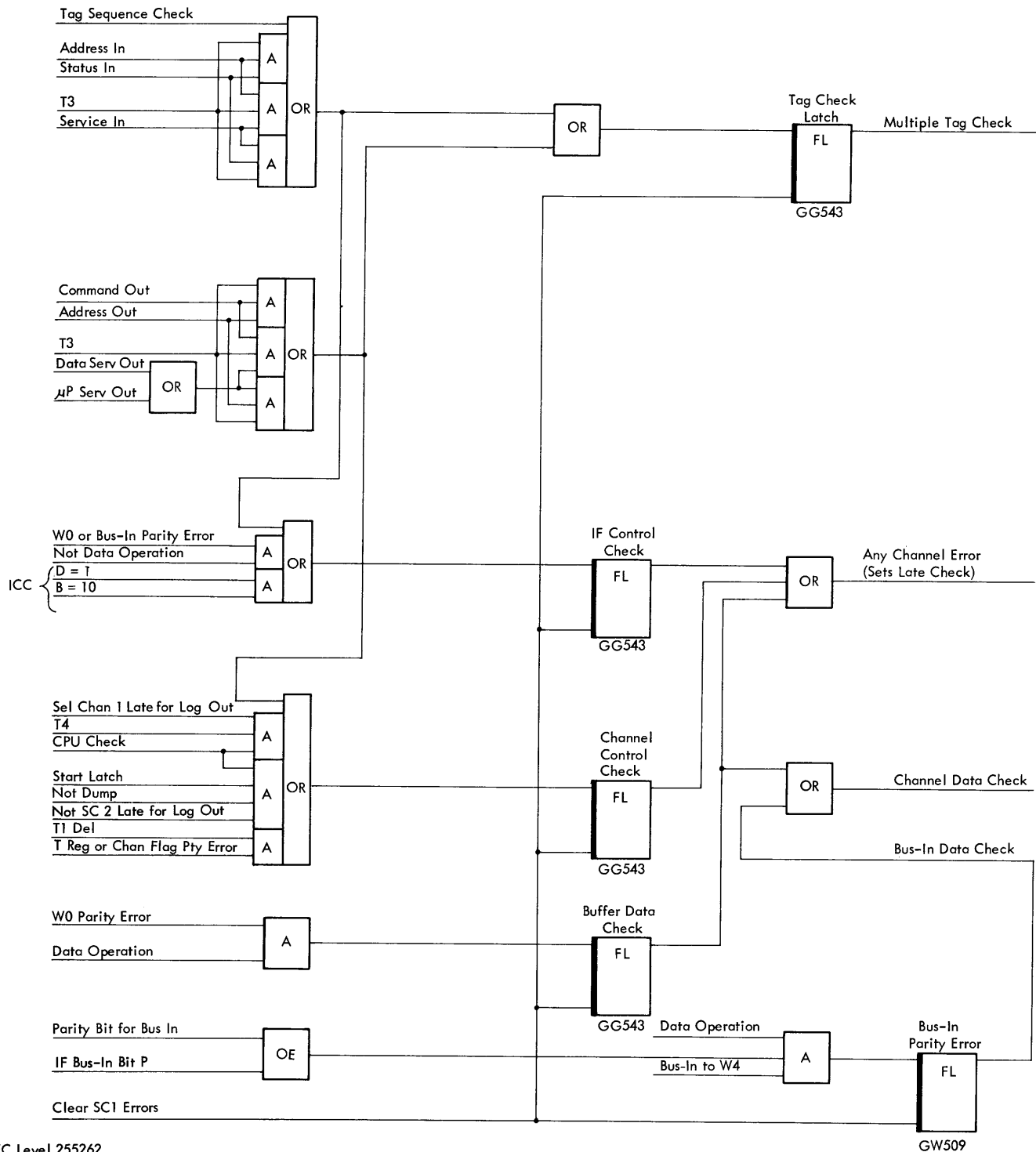
Figure 62. Selector Channel Errors
