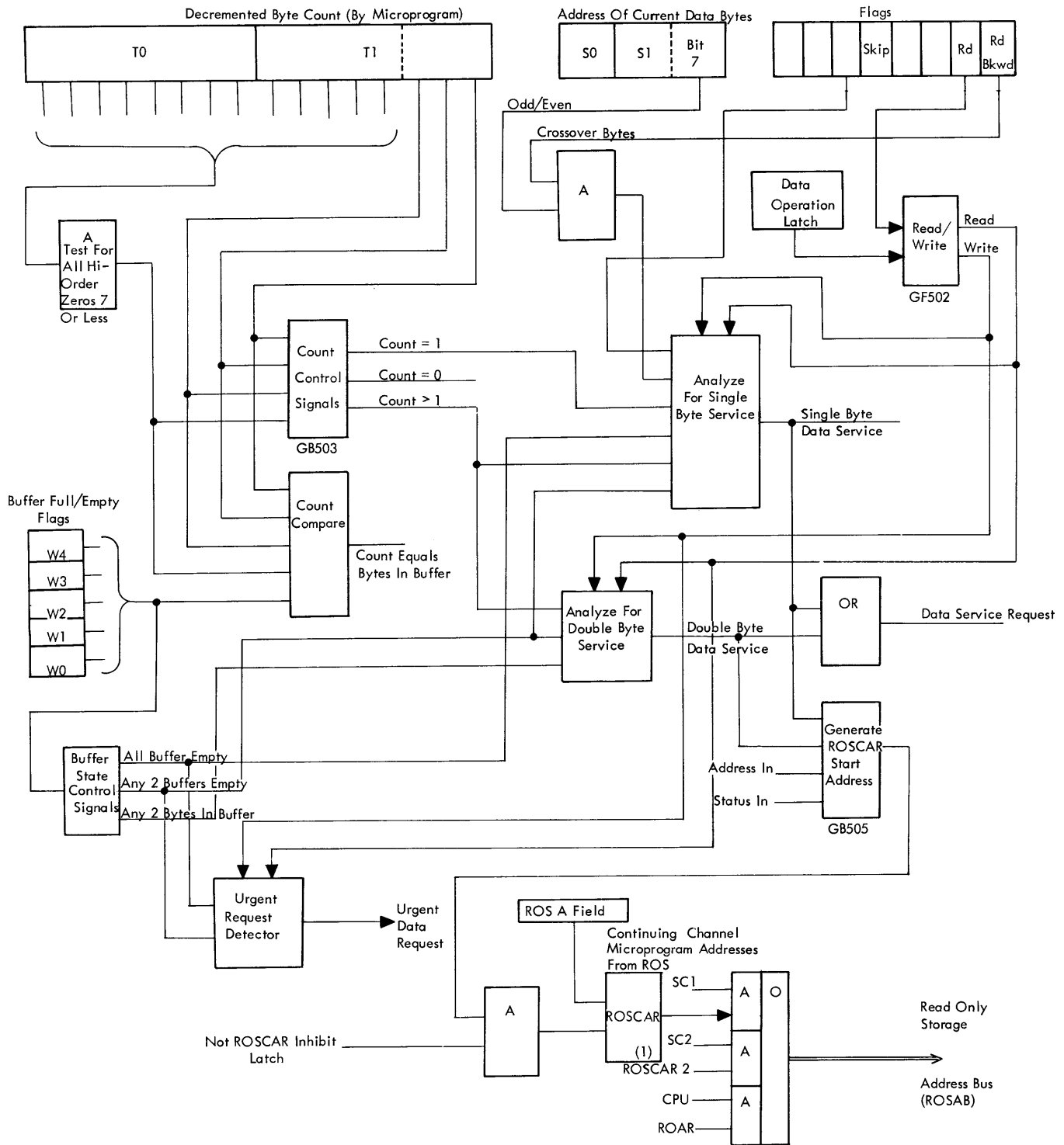
Figure 48. Count Control
