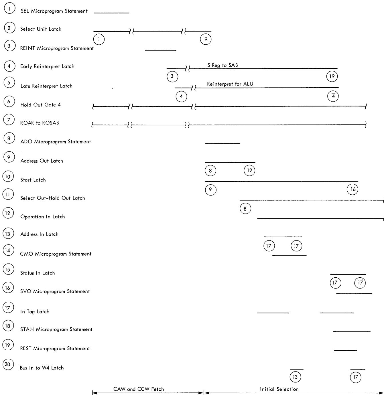
● Figure 41. Start I/O Selector Channel (Sheet 3 of 3)
