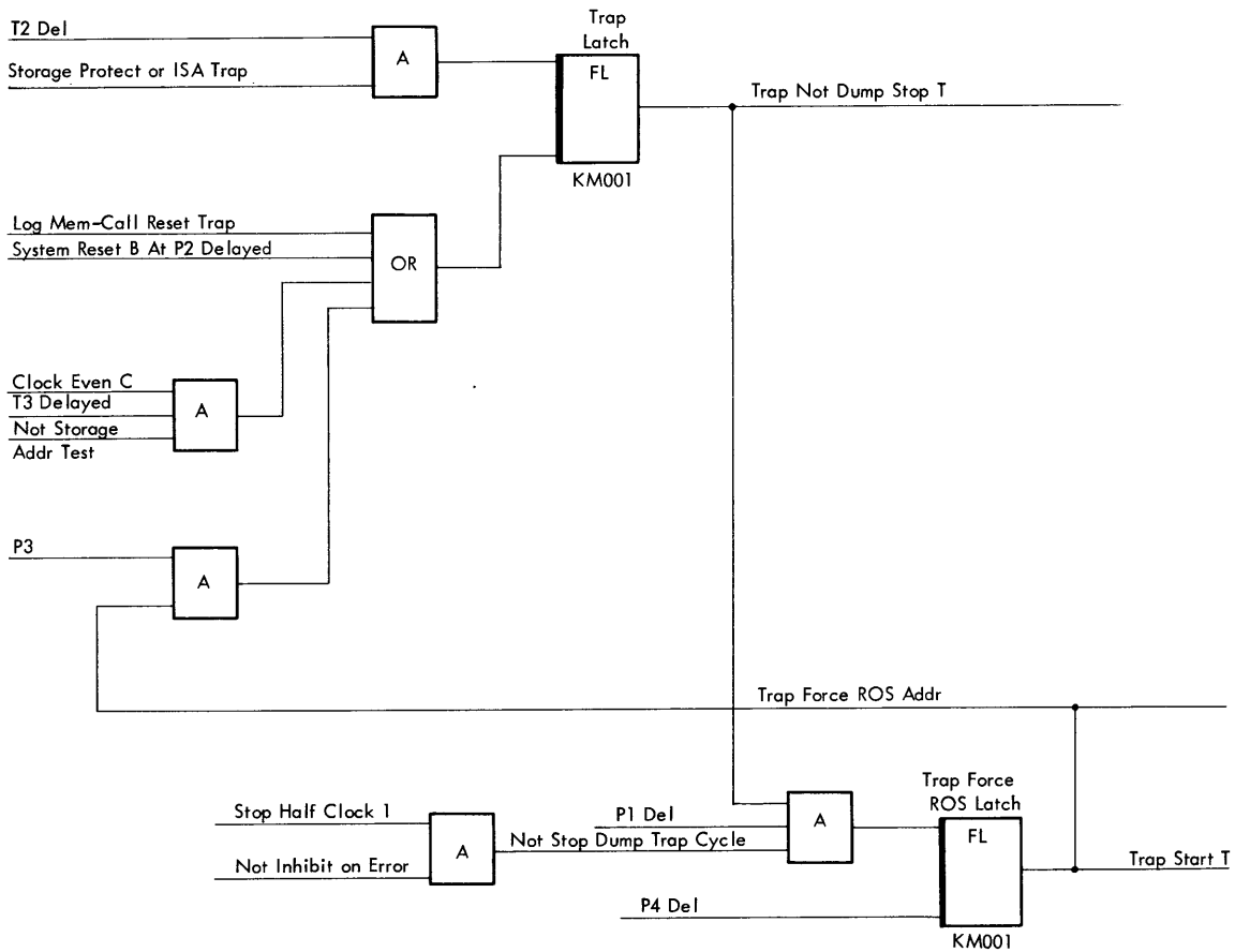
Figure 4. Trap Latch
