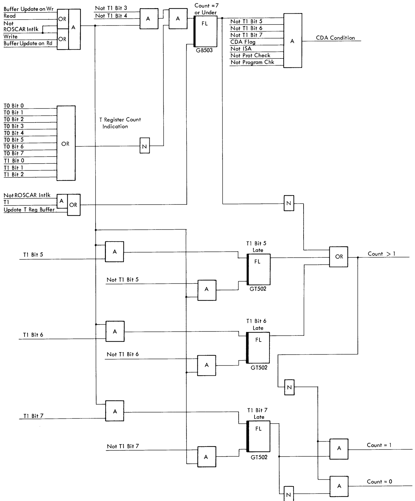
Figure 49. Count Controls
