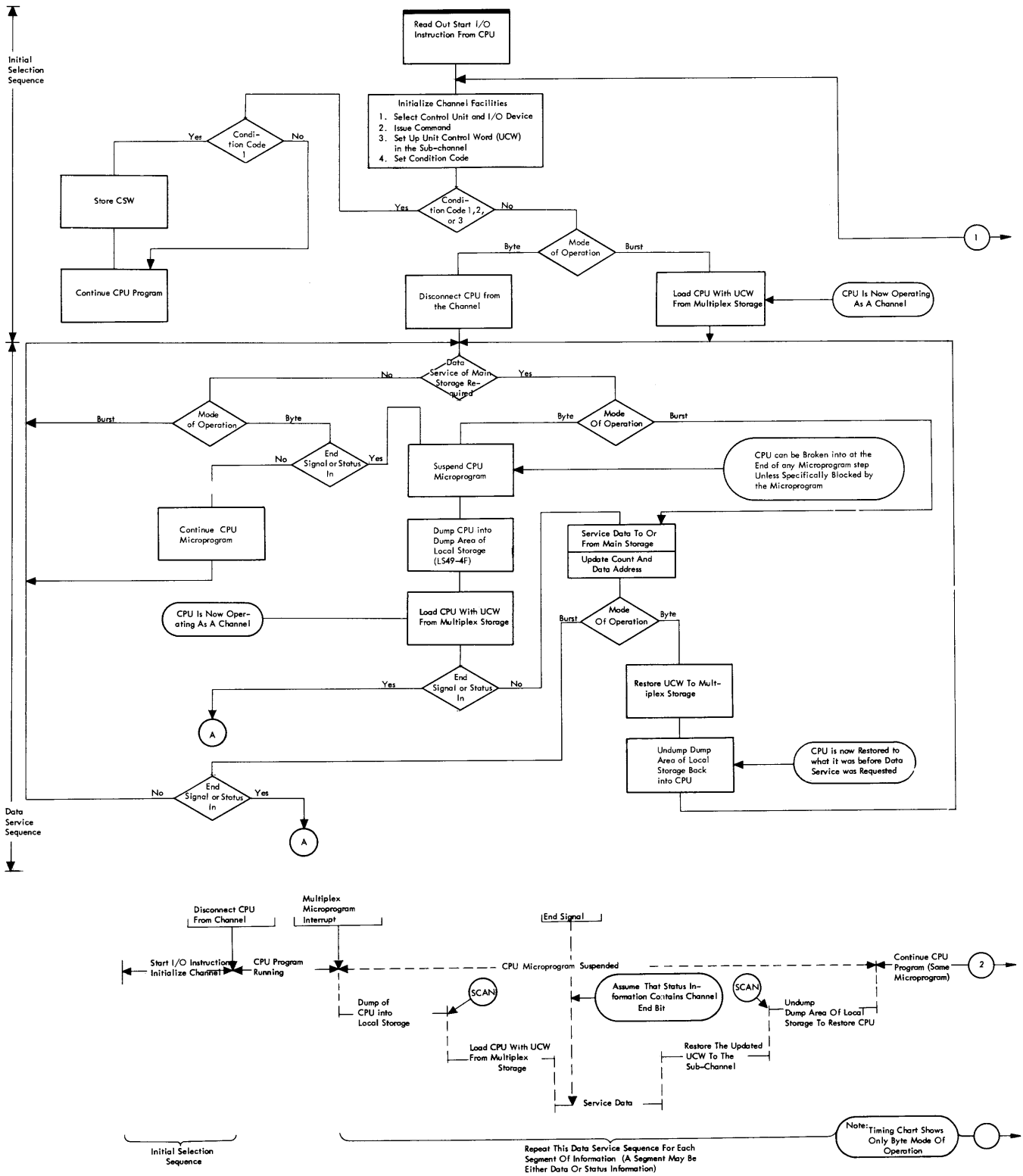
Figure 17. Multiplex Channel Normal Operation (Sheet 1 of 2)
