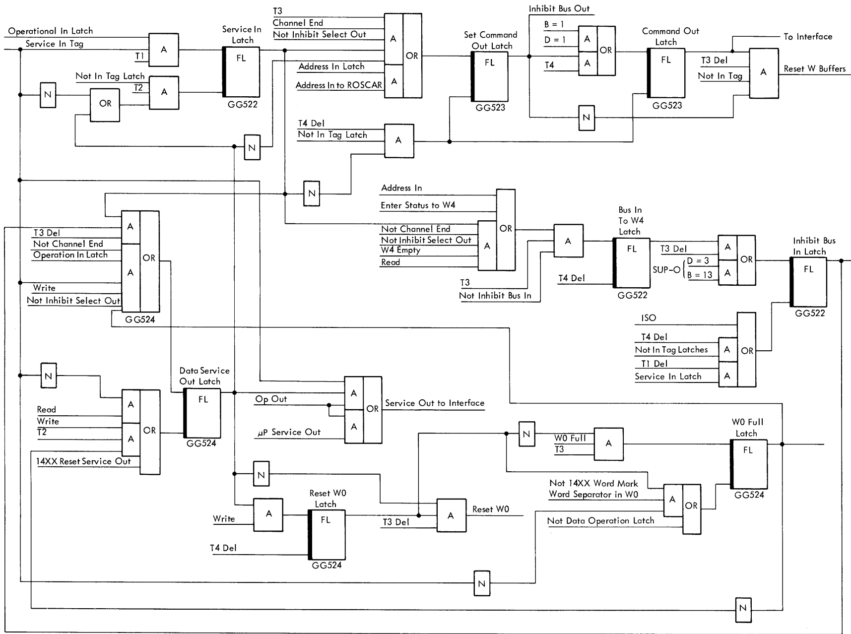
● Figure 43. Data Servicing
