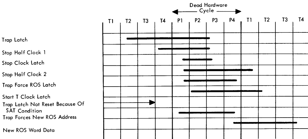
Figure 5. Trap Timing
