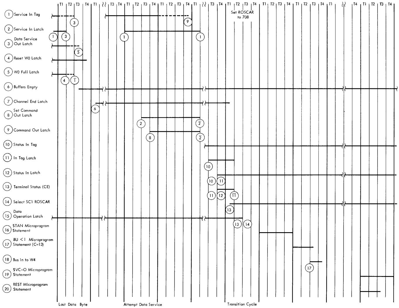
● Figure 58.1 Terminal Status-Write Command
