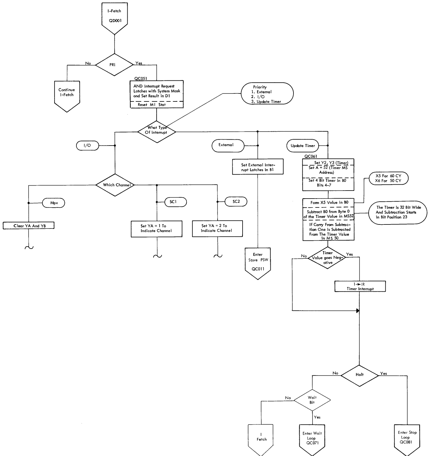
Figure 11. Update Timer
